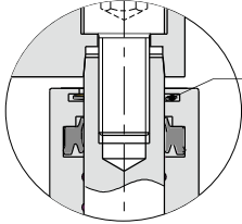
Stainless steel dust scraping ring
