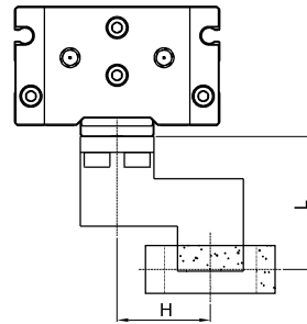
The range of the Opened gripping points
